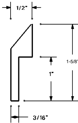
MAXI-TIP 1 and MAXI-TIP 2
