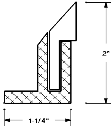
MAXI-TIP or MAXI-TIP II Shown in BLADE HOLDER
