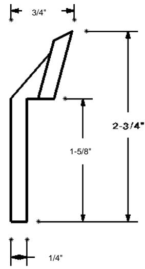
MT Dual Durometer Rigid Base w/ Flexible Tip
